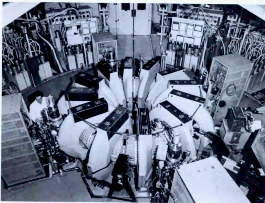
ZT-40M, the latest Los Alamos reversed-field pinch experiment. Toroidal and poloidal current windings are wound on the outer surface of the torus. The large objects surrounding the torus at several positions are the iron transformer cores.
